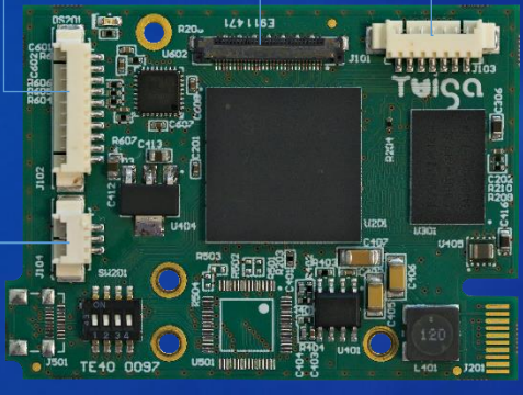
J101 Tamron LVDS Camera Input
